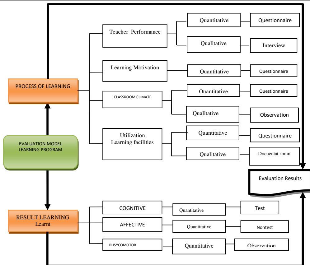
Gambar 1. Model EPH
